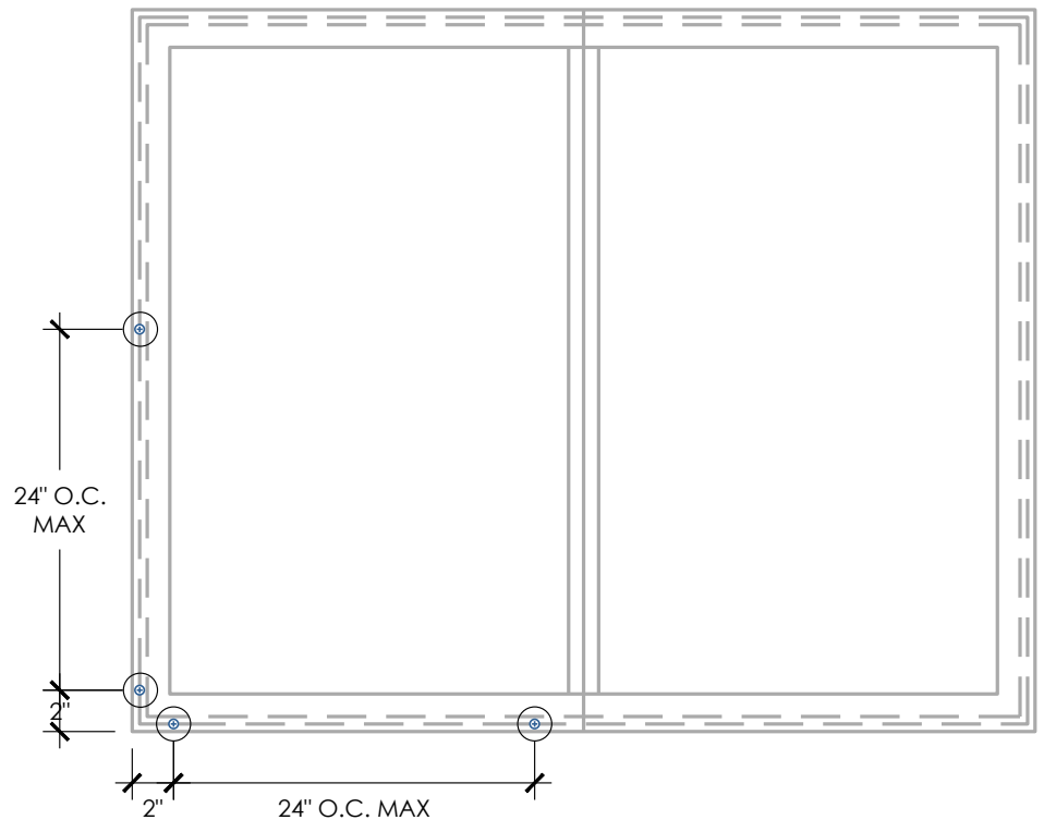
2.0 Screw locations
