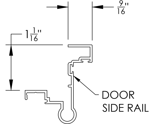
SRF-22 2" x 2" FRAME
