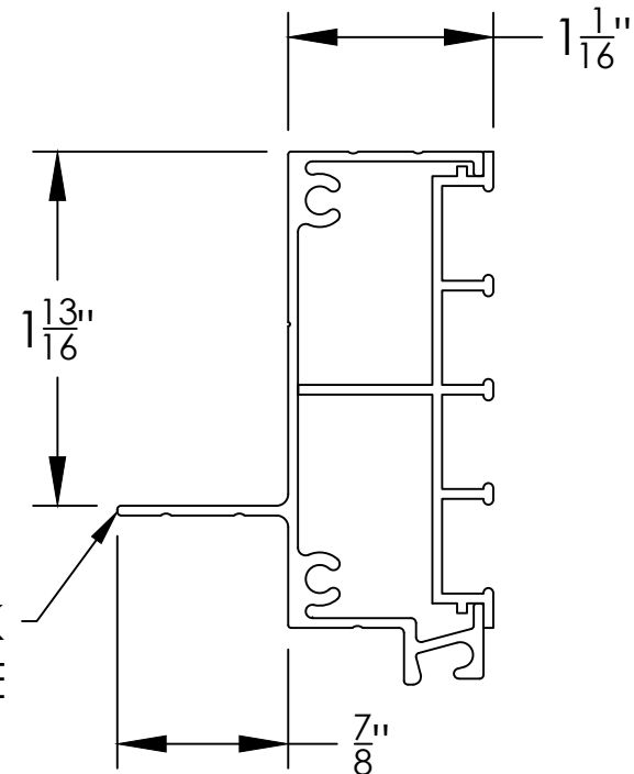
4-TRACK FRAME
