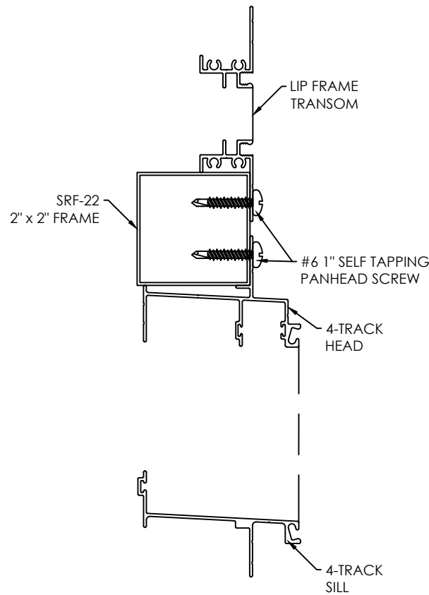
Operable window w/ muller transom
