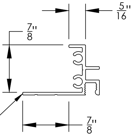
LIP FRAME WINDOW
