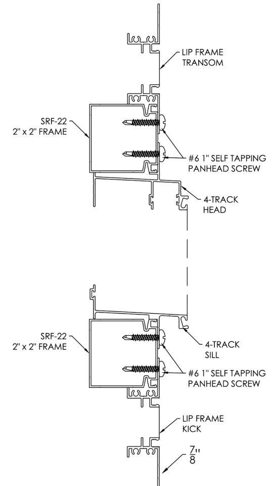
Operable window w/ muller kick and muller transom
